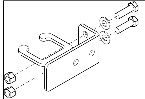
Control Mount Bracket (70048)
